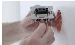
03 Connect the DALI PCU to the pushbutton.
